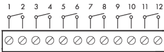
Electrical diagram Relay output
