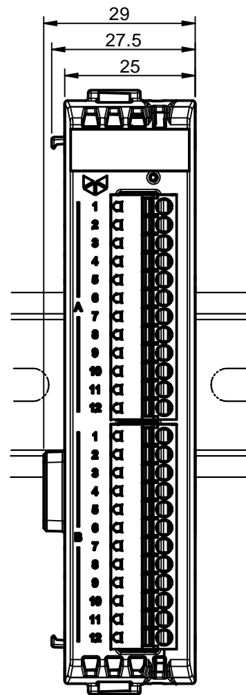
Front view
