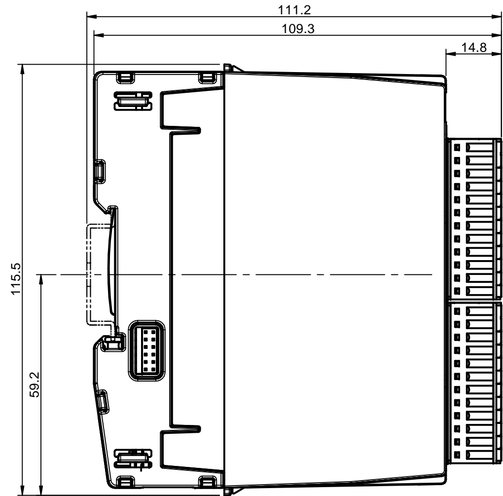
Right view
