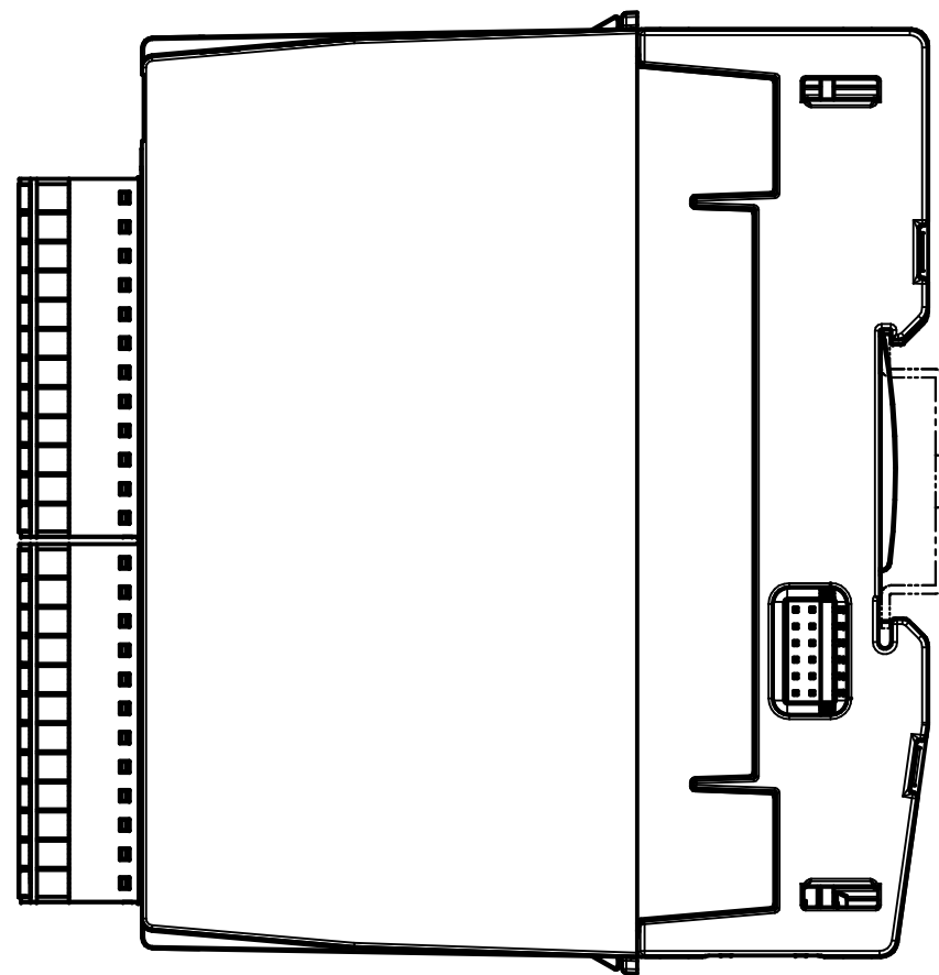
Left view
